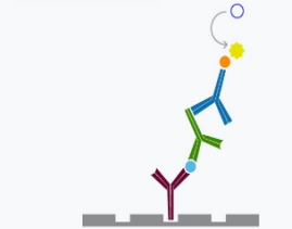
SANDWICH ELISA
